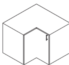
BI FOLD SINK BASE CABINET CODE SIZE mm (W) 935-SI_C2_S_MP-FO_7S 935
