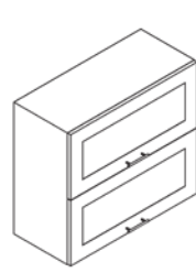
DOUBLE SHUTTER FLAP GALZED WALL CABINET CODE WF2_DF_G_720-FO_7S SIZE mm (W) 600, 800, 900, 1000, 1200
