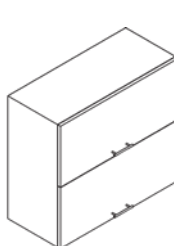
DOUBLE SHUTTER FLAP SOLID HOOD WALL CABINET CODE F2_S_H_720-FO_7S SIZE mm (W) 600, 800, 900, 1000, 1200
