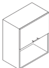
OPEN SOLID FLAP WALL CABINET CODE WFL_PL_S_720-FO_7S SIZE mm (W) 600, 800, 900, 1000, 1200
