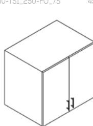
DOUBLE SHUTTER WALL CABINET CODE WS2_600-FO_7S SIZE mm (W) 600, 900, 1000, 1200 WS2_720-FO_7S WS2_960-FO_7S
