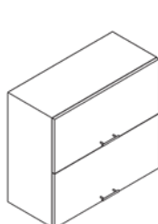
DOUBLE SHUTTER FLAP SOLID WALL CABINET CODE WF2_S_600-FO_7S SIZE mm (W) 600, 800, 900, 1000, 1200
