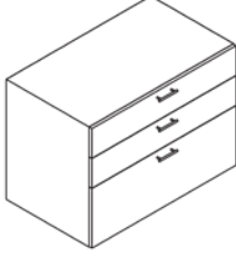
TRIPPLE DRAWER BASE CABINET FOR HOB CODE SIZE mm (W) BS_D3_2EQ_TB-FO_7S 450, 500, 600, 800 900, 1000, 1200
