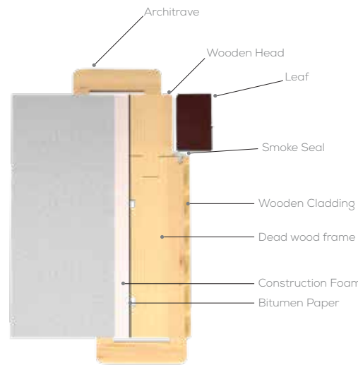
ENGINEERED JAMB FRAME (WITH CLADDING)
