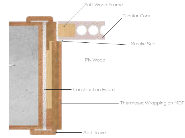
PLY WOOD JAMB FRAME
