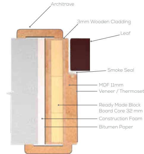
VENEERED JAMB FRAME (VENEERED, THERMOSET & PAINTED)
