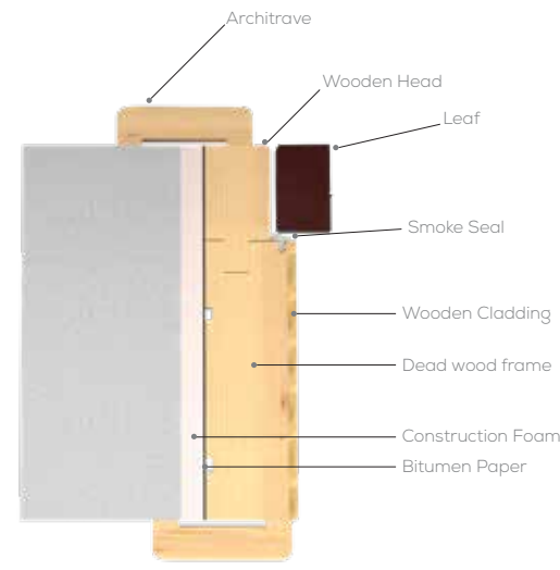
ENGINEERED JAMB FRAME (WITH CLADDING)
